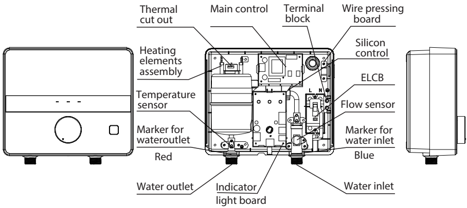
↑ PRODUCT STRUCTURE FOR TWH-65EGNTH(K)
