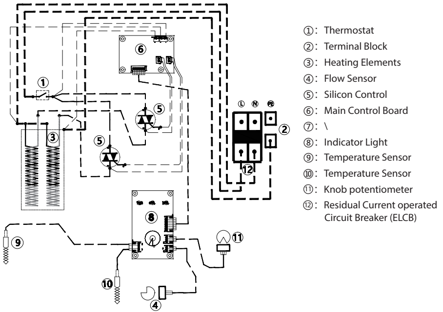
WIRING DIAGRAM FOR TWH-65EGNTH(K)
