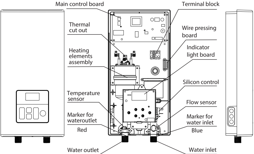
↑ PRODUCT STRUCTURE FOR TWH-**EFNTH(W)-CB
