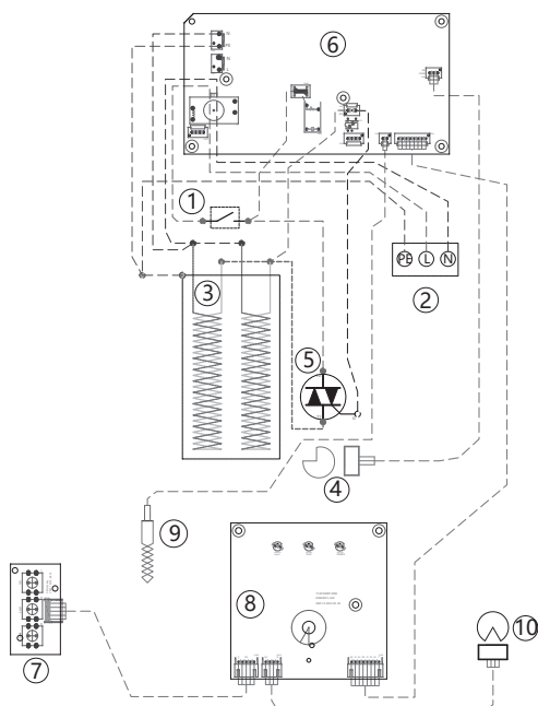
WIRING DIAGRAM FOR: TWH-**MFNTH(W)-WB
