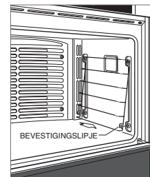
Ovenrekgeleiders
