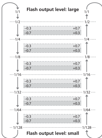
Selector dial rotated counterclockwise
