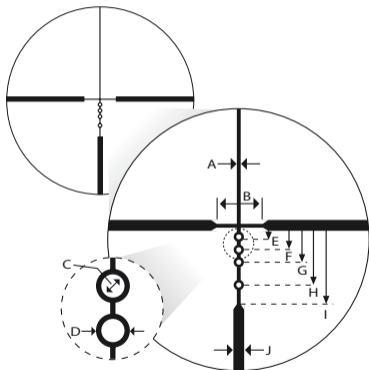
BDC 150 reticle
