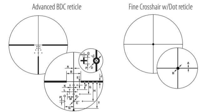
Letters A to P in the diagram above refer to the reticle subtensions of units A to P shown on the table to the right.
