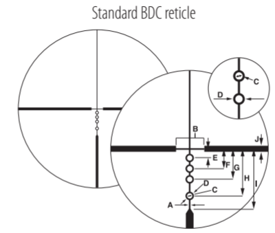
Letters A to J in the diagram above refer to the reticle sub-tensions of units A to J shown on the table to the right.
