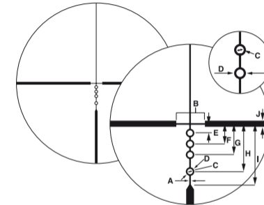
Standard BDC reticle
