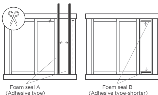
Sliding Window Installation
