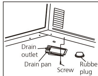
Bottom drainage
