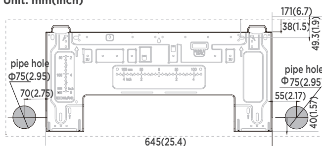
Indoor unit dimensions(WxH): 1000mm(39.37in)x335mm(13.19in)
