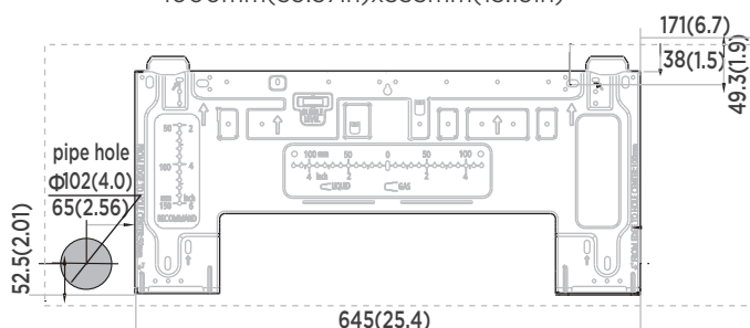
Indoor unit dimensions(WxH): 1000mm(39.37in)x335mm(13.19in)
