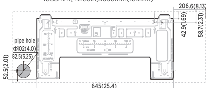
Indoor unit dimensions(WxH): 1088mm(42.83in)x336mm(13.22in)
