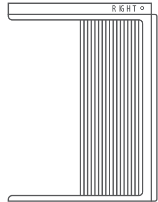
Frame Assembly(Right)
