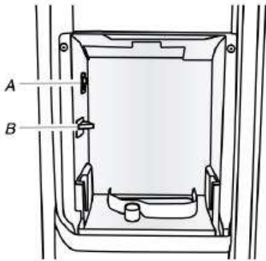
A. On/Off switch B. Storage bin sensor
