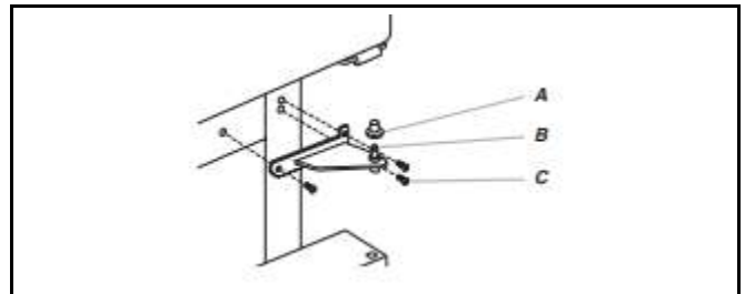
A. Hinge Pin Cover C. Hinge Screws B. Bottom Hinge
