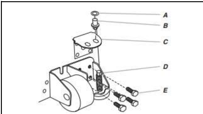
A. Hinge Pin Shim D. Roller Bracket B. Bottom Hinge E. 3/8" Hex-Head Screws C. Hinge Plate
