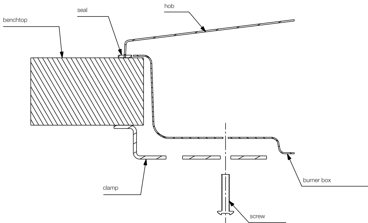
Figure 7 – Clamp fitment
