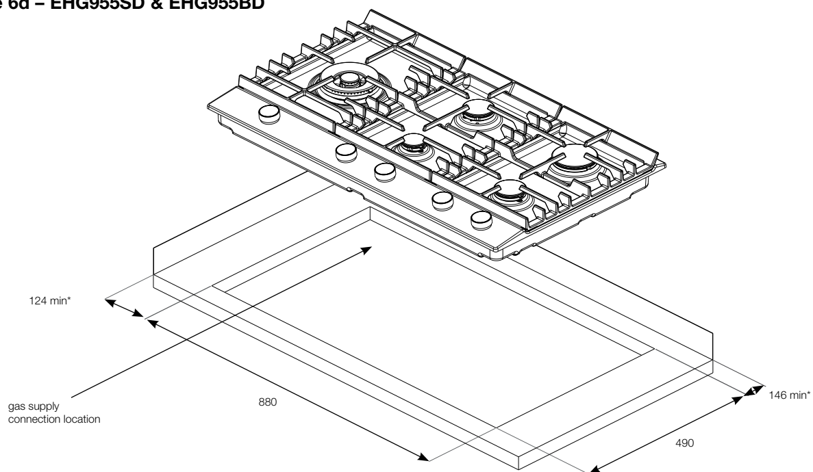
Figure 6d – EHG955SD & EHG955BD
