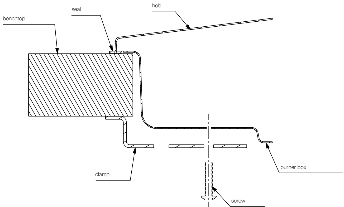
Figure 7 – Clamp fitment
