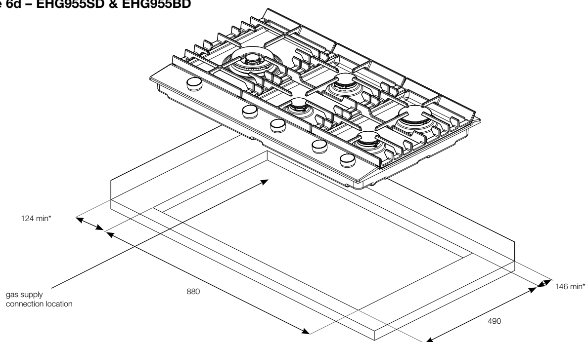
Figure 6d – EHG955SD & EHG955BD
