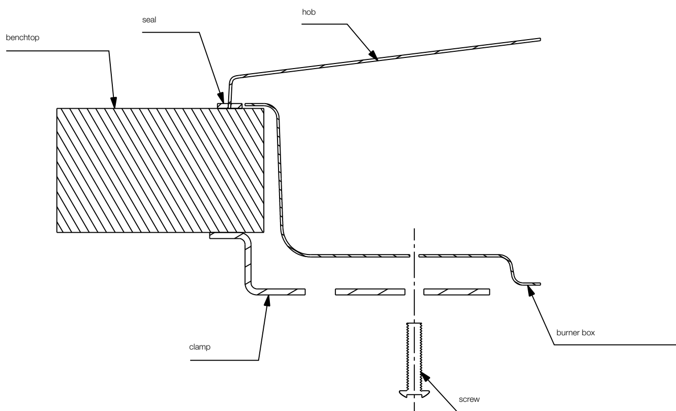
Figure 8 – Clamp fitment
