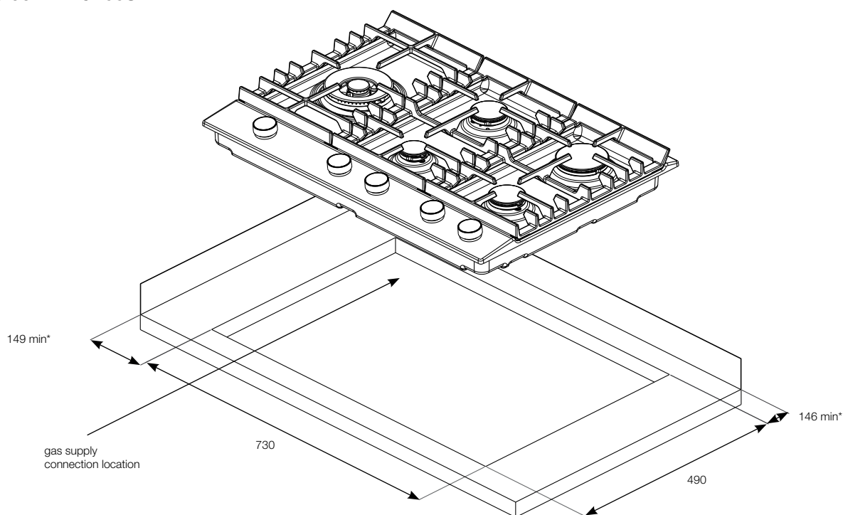
Figure 6c – EHG755SD
