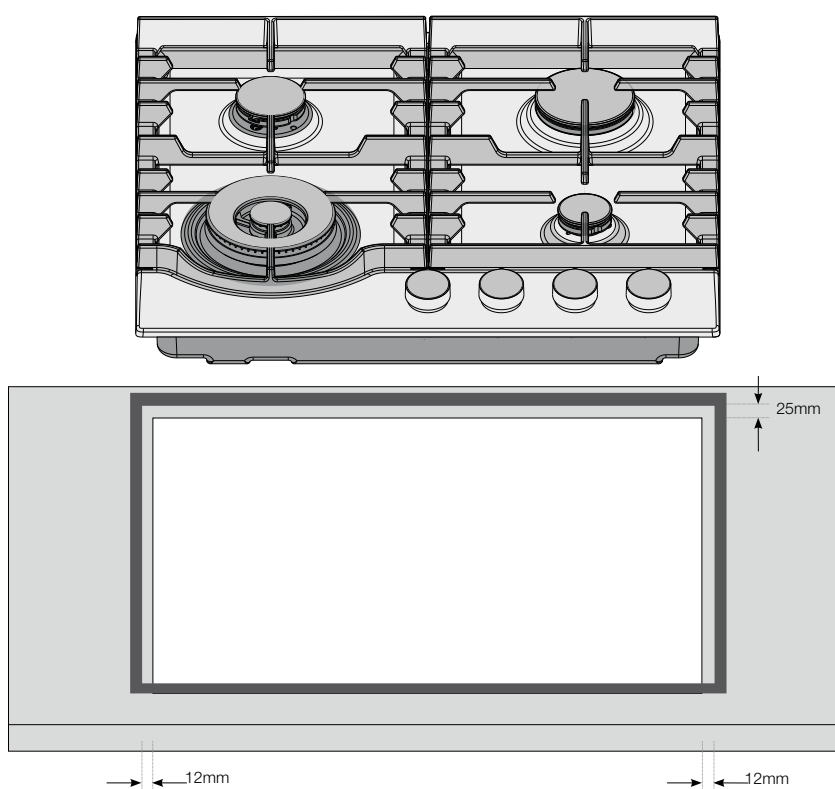
Figure 8a - Mastic seal position for model EHG645SD
