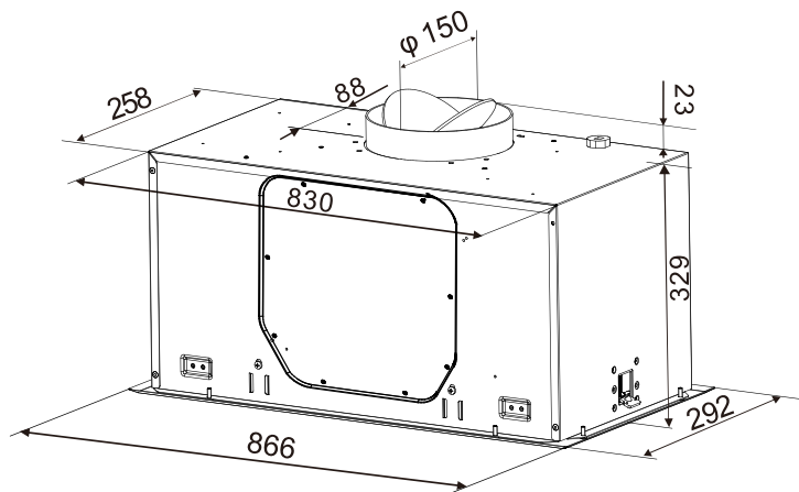
Product dimensions for ERI955DSE
